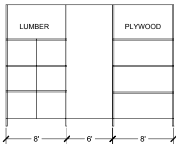
RACK ELEVATION A
